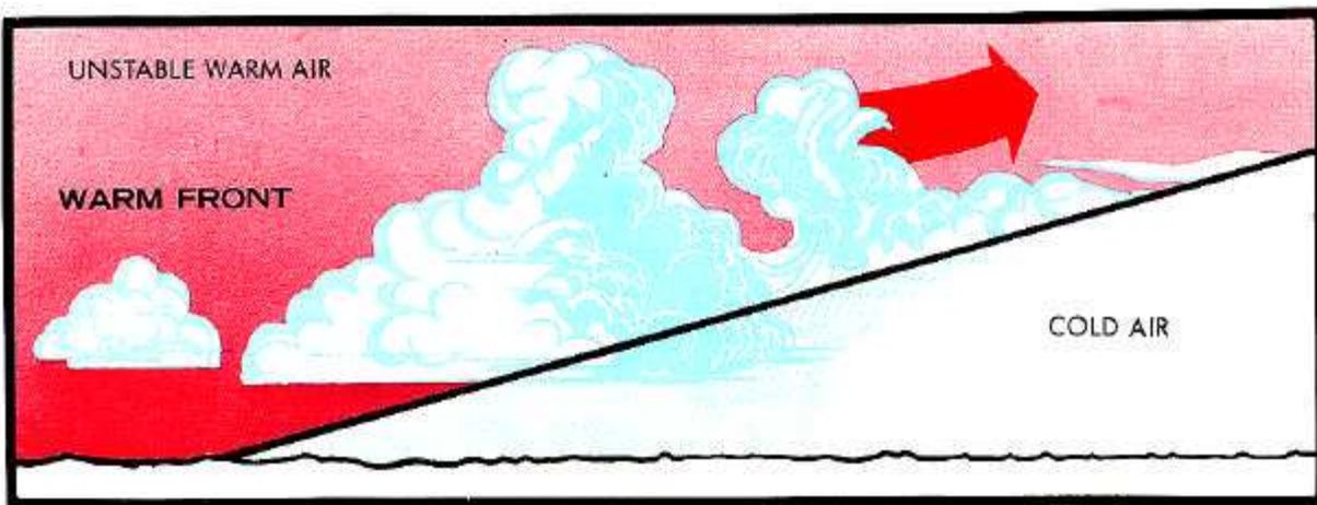
If the warm air above a warm front is moist and conditionally unstable, altocumulus and cumulonimbus clouds form. Often, thunderstorms will be embedded in the cloud masses.
