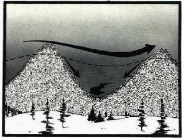
A nighttime inversion in a valley effectively shields the downslope and downvalley winds from the general wind flow above.
