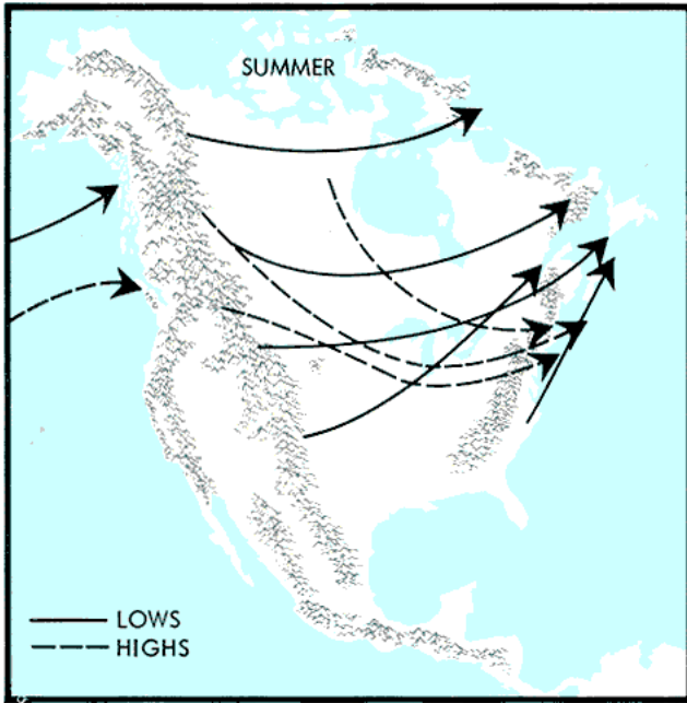
In the summer the preferred tracks of migratory Lows and Highs are rather far north, mostly across Southern Canada or the Northern States. A few Lows travel northeastward along the Atlantic coast.
