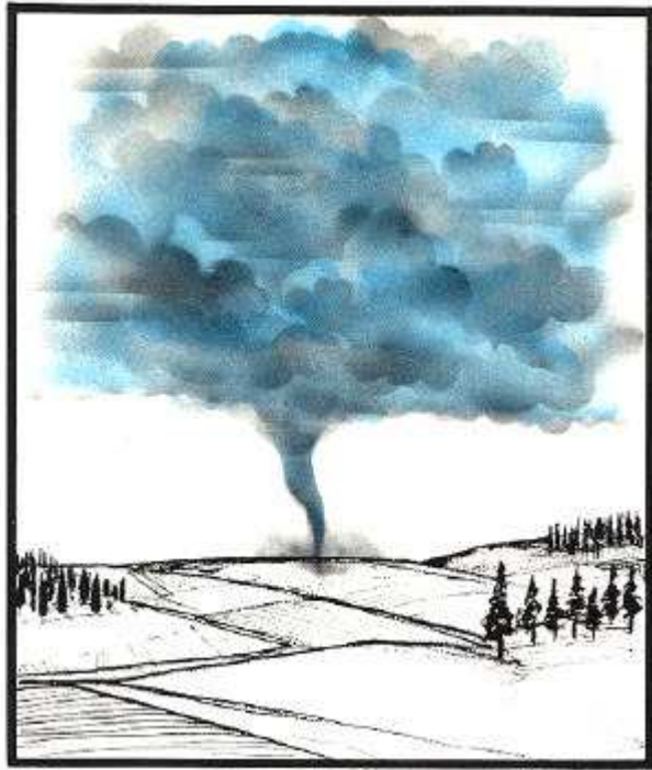
A tornado is a violently whirling vortex which occurs with a severe thunderstorm. The rotating tube builds downward from the cumulonimbus cloud. Destruction results from extremely strong wind and low pressure.
