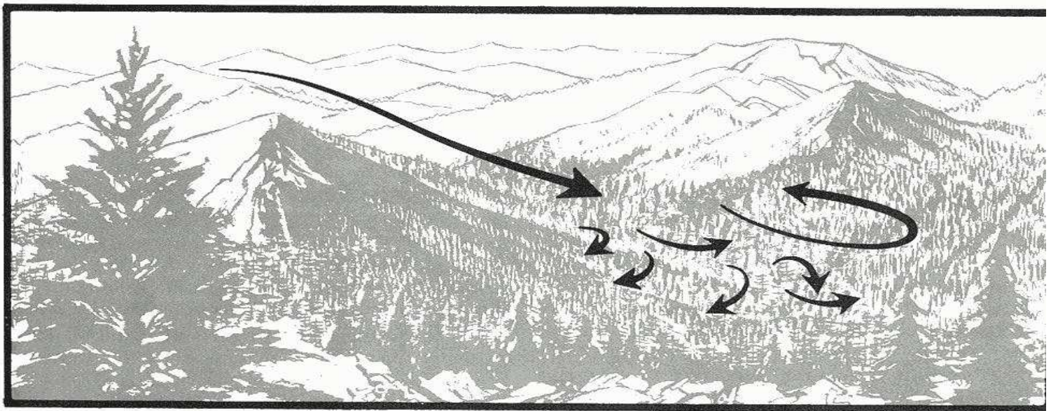
Ridgetop saddles and mountain passes form important channels for general wind flow. The flow converges and the wind speed increases in the passes. Horizontal and vertical form on the lee side of saddles.
