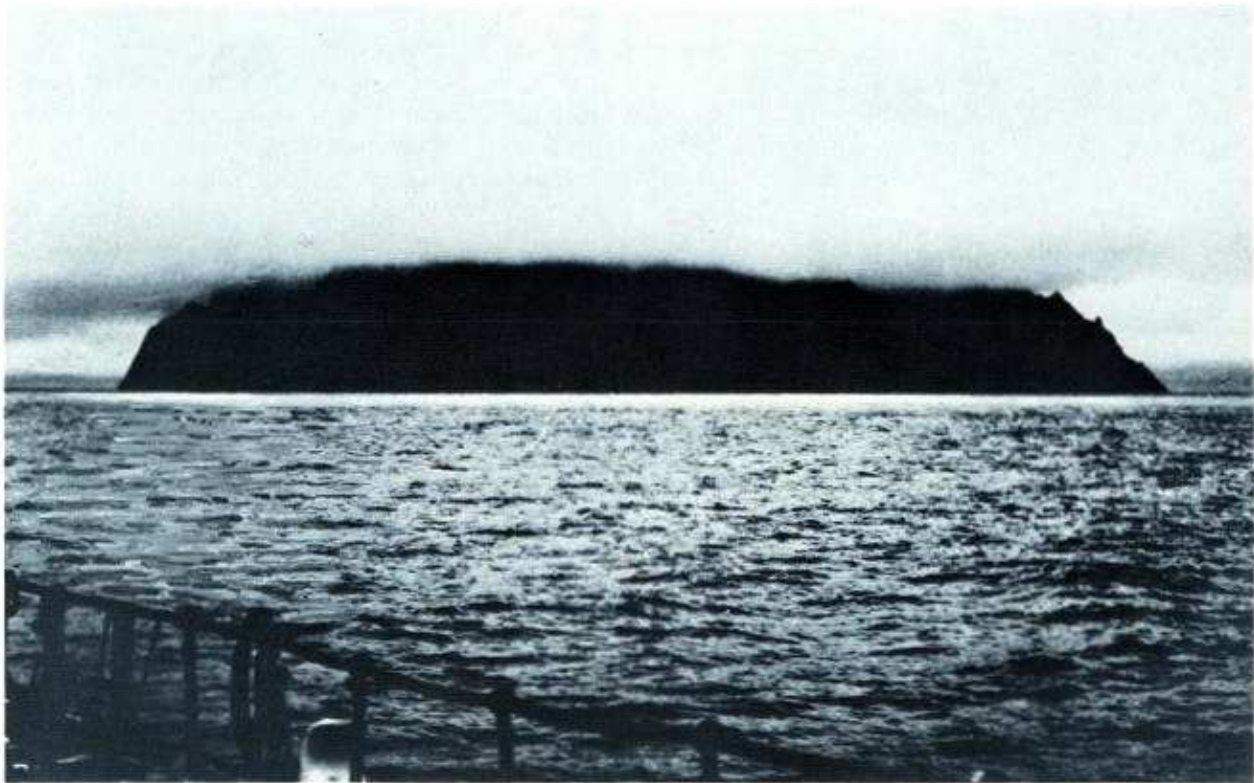
Stratus is a low, gray cloud layer with a fairly uniform base and top. Usually it does not produce precipitation, although it may cause some drizzle or snow grains. Stratus often forms by the lifting of a layer of fog.
