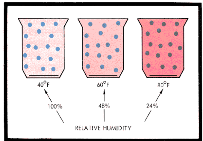
Relative humidity decreases as temperature increases even though the amount of water vapor in the air remains the same.
