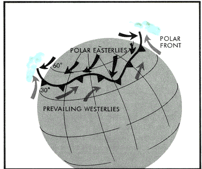
The polar front zone is an area of storminess, cloudiness, and precipitation, and its position is extremely variable.
