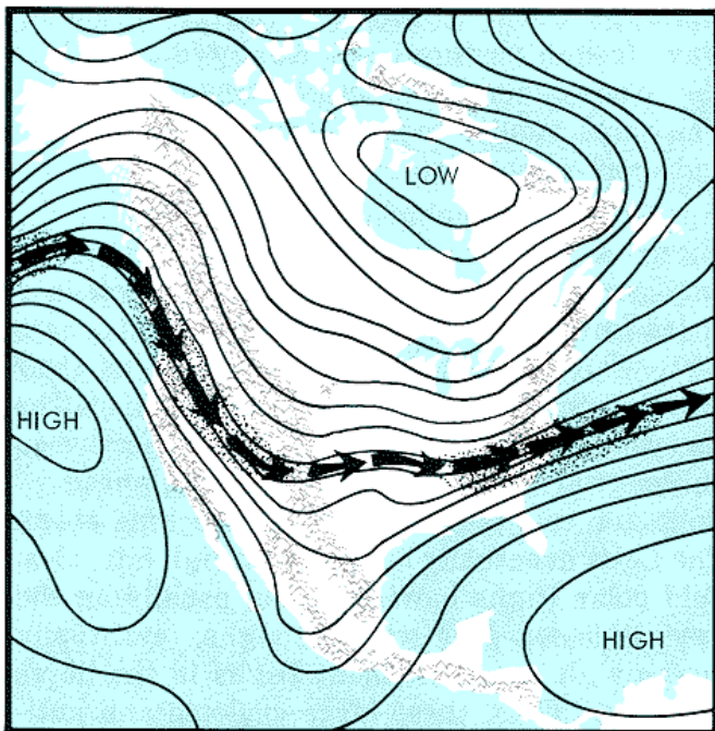
The jet stream, as shown on a constant-pressure chart in the upper troposphere, is meandering, fast-flowing river of air embedded in the belt of westerlies. The stippling shows the regions of strongest winds that move along the jet stream.
