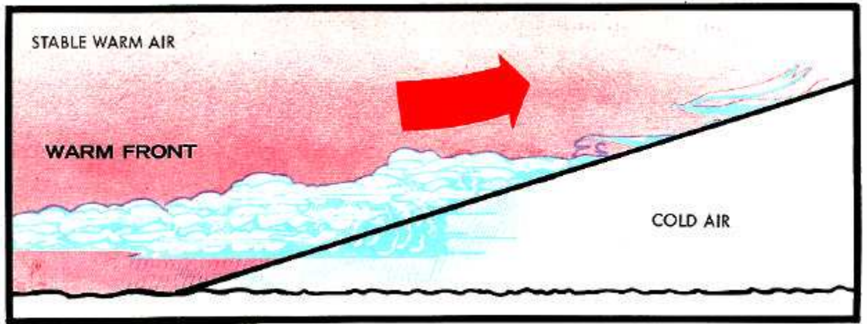
If the warm air above a warm front is moist and stable, clouds are of the stratus type. The sequence of cloud types is cirrus, cirrostratus, altostratus, and nimbostratus. Precipitation is steady and increases gradually with the approach of a front.
